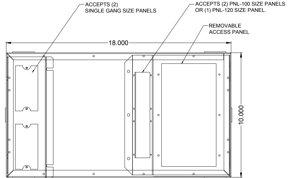
2 TOP VIEW BACK BOX
