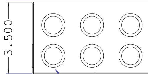
(6) 1/2", 3/4" COMBINATION KNOCKOUTS. TYPICAL ON OPPOSING SIDES
